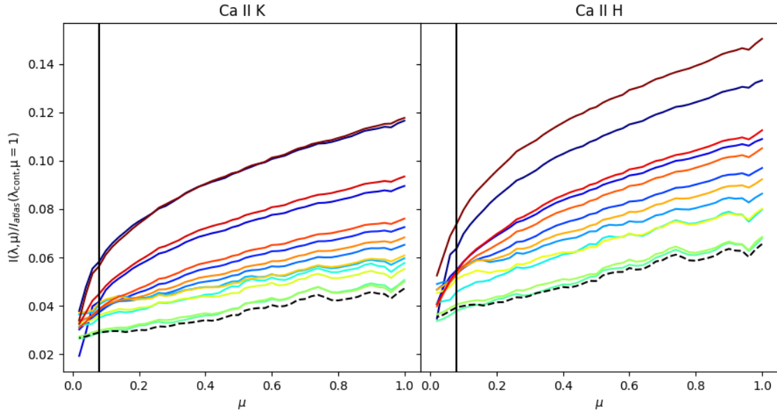
Fig. 5. An enlarged version of the first two panels in the left column of Fig. 4.
