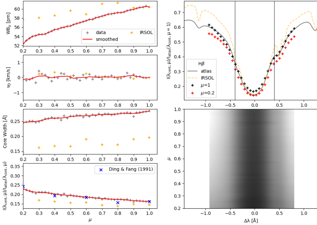
Fig. 15. Left: Four panels showing the bound equivalent width, line shift, core width, and line depth, respectively. Right: The representative profiles of H \beta . In the upper panel we plot a convolved profile from the solar atlas as well as our data at \mu = 1 and \mu = 0.2 . The lower panel shows a 2D representation of all 50 profiles.
