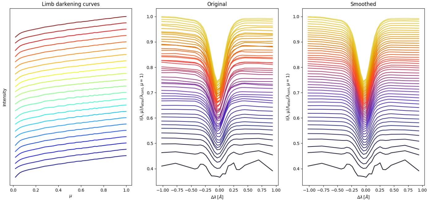
Fig. 3. Comparison of normalized average OI 7772 Å profiles before and after smoothing to remove effects from p-modes. Left: The un-smoothed limb darkening data of each wavelength point in the OI 7772 Å line on an arbitrary intensity scale. The curves are ordered by wavelength, with the top (red) curve representing the red continuum, the middle (green) curve representing the line core, and the bottom (blue) curve representing the blue continuum. The oscillatory behavior is most pronounced around the line core (green), between a \mu of 0.3 to 0.8. Middle: The original representative profiles, ranging from \mu = 1 to \mu = 0.02 . The profile representing \mu = 1 is shown in yellow at the top of the figure, with each consecutive profile beneath it in a different color. Right: Same as the middle panel, but with most of the p-mode effects removed after limb darkening curves were smoothed.
