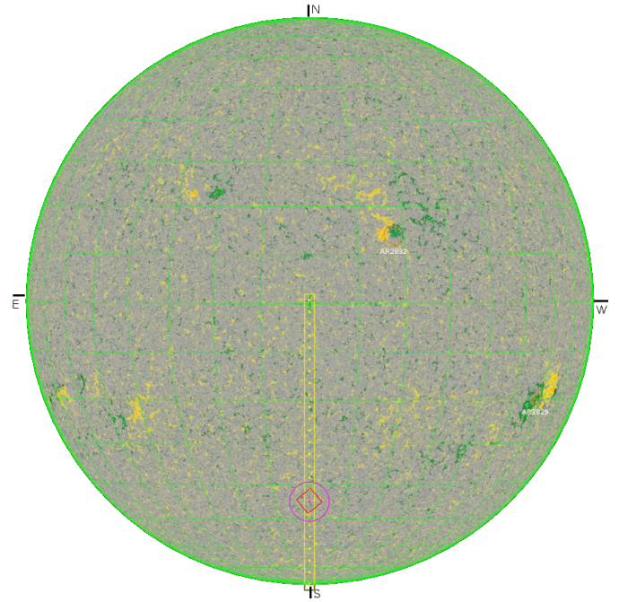
Fig. 1. Screen capture of the primary image guider of the SST showing the HMI magnetogram with 25 pointings in a mosaic that spans from the solar south pole to the disk center, taken on the 12th of June 2021. The red marker represents the location that the telescope was aimed at, at the moment that the image was taken.
