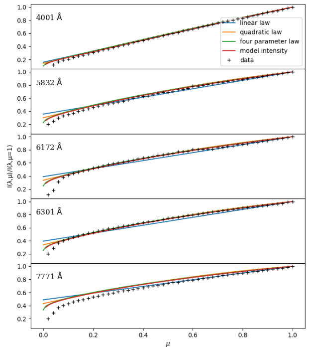
Fig. 7. Limb darkening as a function of \mu compared to the intensity variation generated for the sun from the ATLAS stellar model (red) and the resulting linear (blue), quadratic (orange) and four parameter (green) limb darkening laws. The model and all three laws generally match the solar limb darkening out to \mu = 0.1 at 4001-6301 Å, but underpredict the limb darkening at 7771 Å. The linear law is the most different from the data at all wavelengths due to its simplicity.
