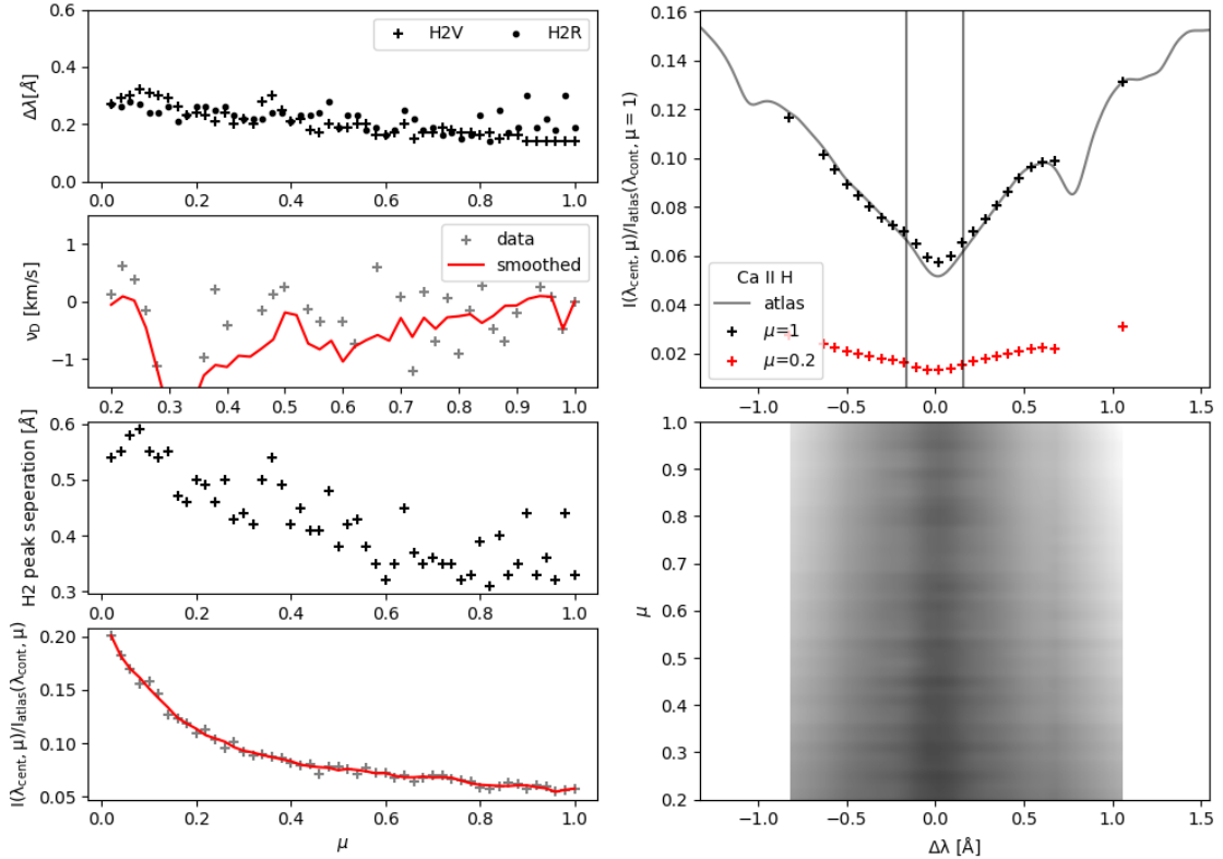
Fig. 14. Same as Fig. 13, but for Ca II H.
