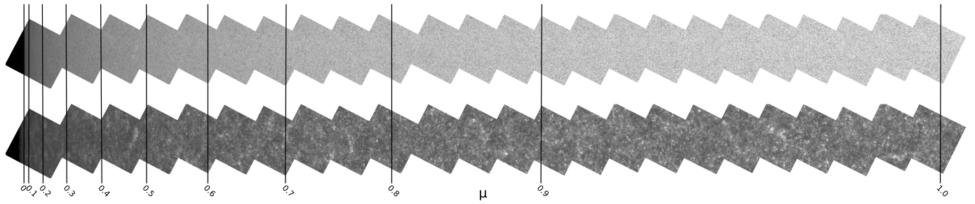
Fig. 2. Overview of mosaics taken during Campaign I, starting from the solar limb on the left and going to disk center on the right. The mosaics span roughly 1000 \times 80 arcseconds. Top: Continuum near blue wing of Fe I 6301 Å. Bottom: Line center of Ca II 8542 Å. It can be seen that the Sun seems to extend past \mu = 0 in the chromosphere.
