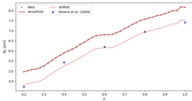
Fig. 8. An enlarged version of the first panel of Fig. 12 showing the equivalent width of the OI 7772 Å line as a function of \mu compared with measured values by Pereira et al. (2009). We plot the data (gray), the smoothed data (red), the measurements of Pereira et al. (2009) (blue), and our smoothed data shifted down to match the disk center observation of the blue points in light red. The latter is added to ease comparison in gradient between the two data sets.
