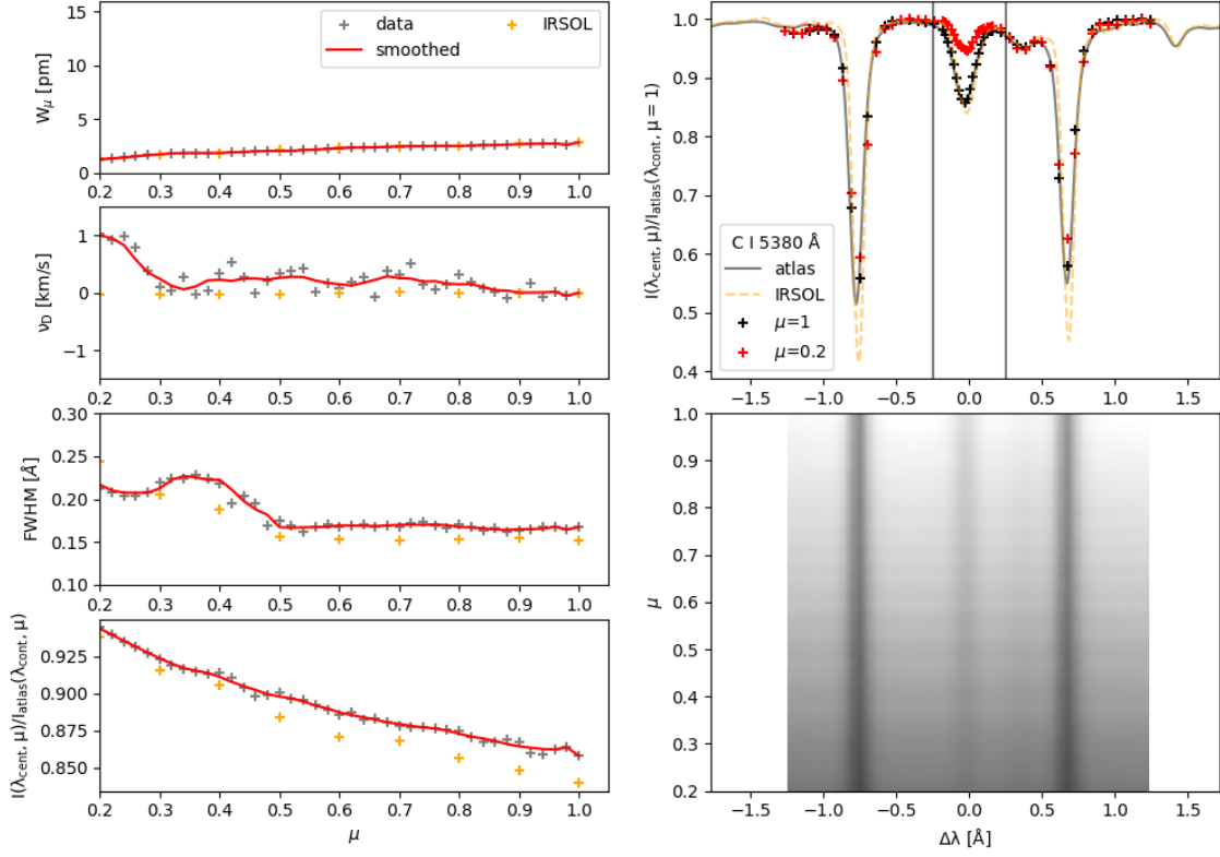
Fig. 9. Left: Four panels showing the equivalent width, line shift, FWHM, and line depth, respectively. Right: The representative profiles of C I 5380 Å. In the upper panel we plot a convolved profile from the solar atlas as well as our data at \mu = 1 and \mu = 0.2 . The pair of black lines show the range over which the equivalent width has been calculated.
