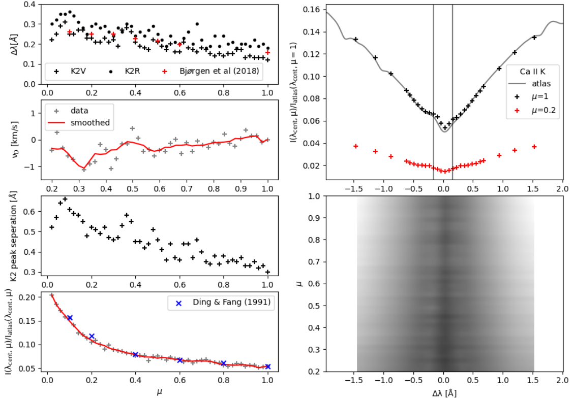
Fig. 13. Left: Four panels showing the K2 peak location, line shift, K2 peak separation, and line depth, respectively. Right: The representative profiles of Ca II K. In the upper panel we plot a convolved profile from the solar atlas as well as our data at \mu = 1 and \mu = 0.2 . The lower panel shows a 2D representation of all 50 profiles.
